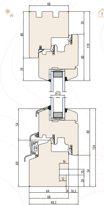
SYSTEM NATURO 68 Innere Fensterbankfräsung
