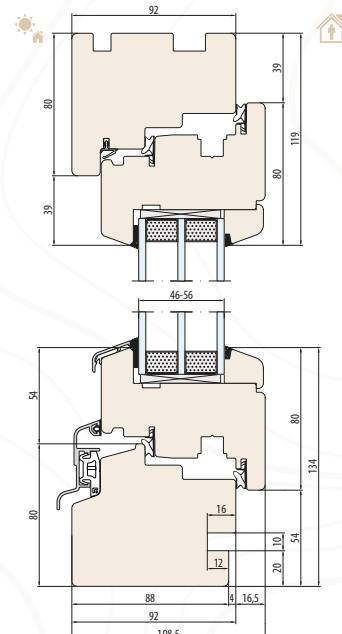
SYSTEM NATURO 92 Innere Fensterbankfräsung
